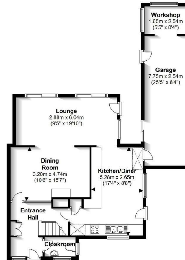
Ground Floor Approx. 88.7 sq. metres (955.3 sq. feet)
